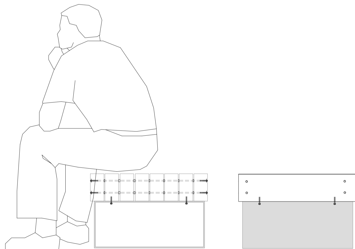
2 TYPICAL DETAIL: SEATING type a 12 SCALE 1:10 @ A1 Materials 6mm Corten steel Module 1 Hardwood Timber slats 140mm x 70 mm x 1000
