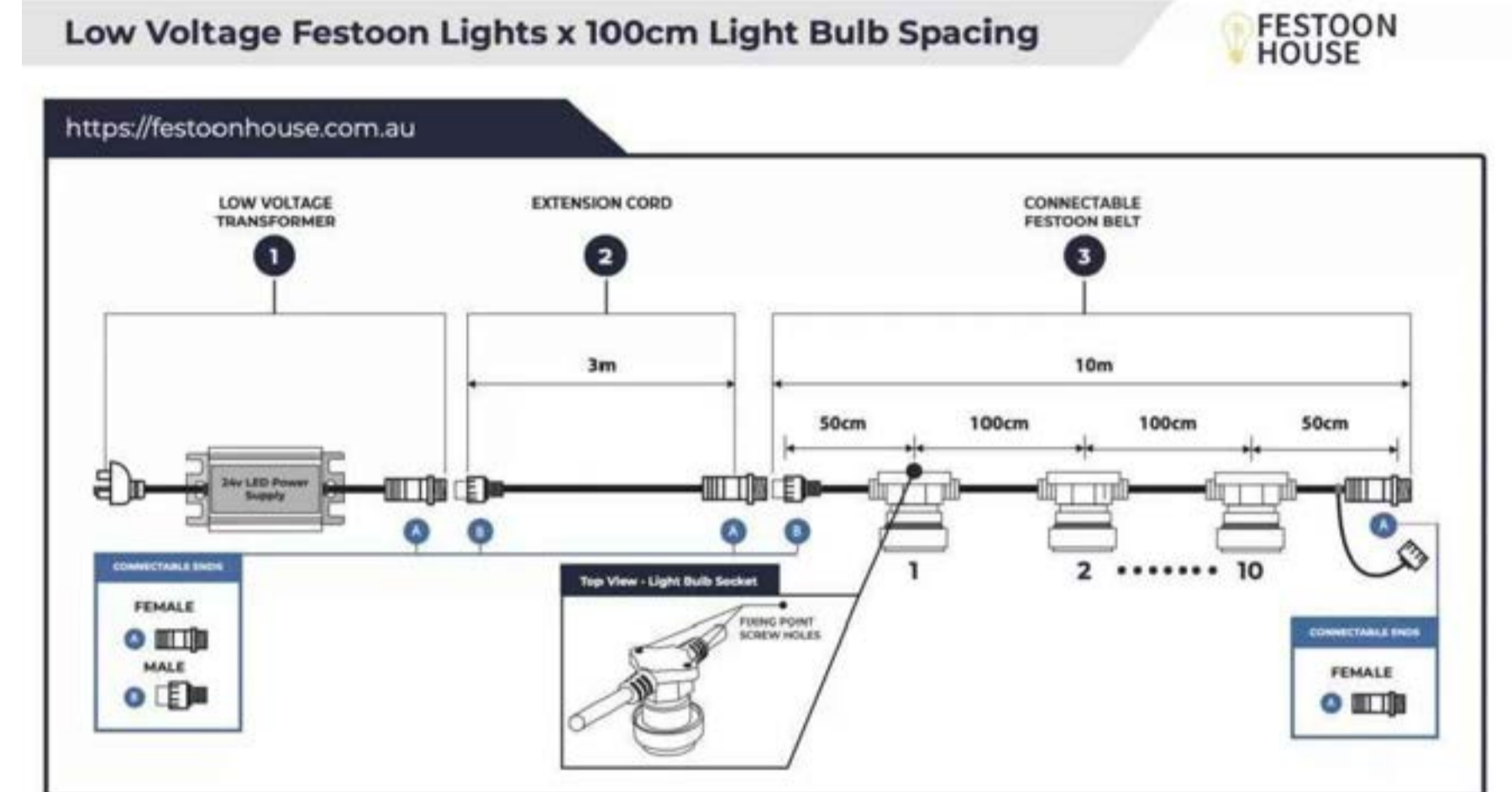
4 Specification Festoon Lights 12
