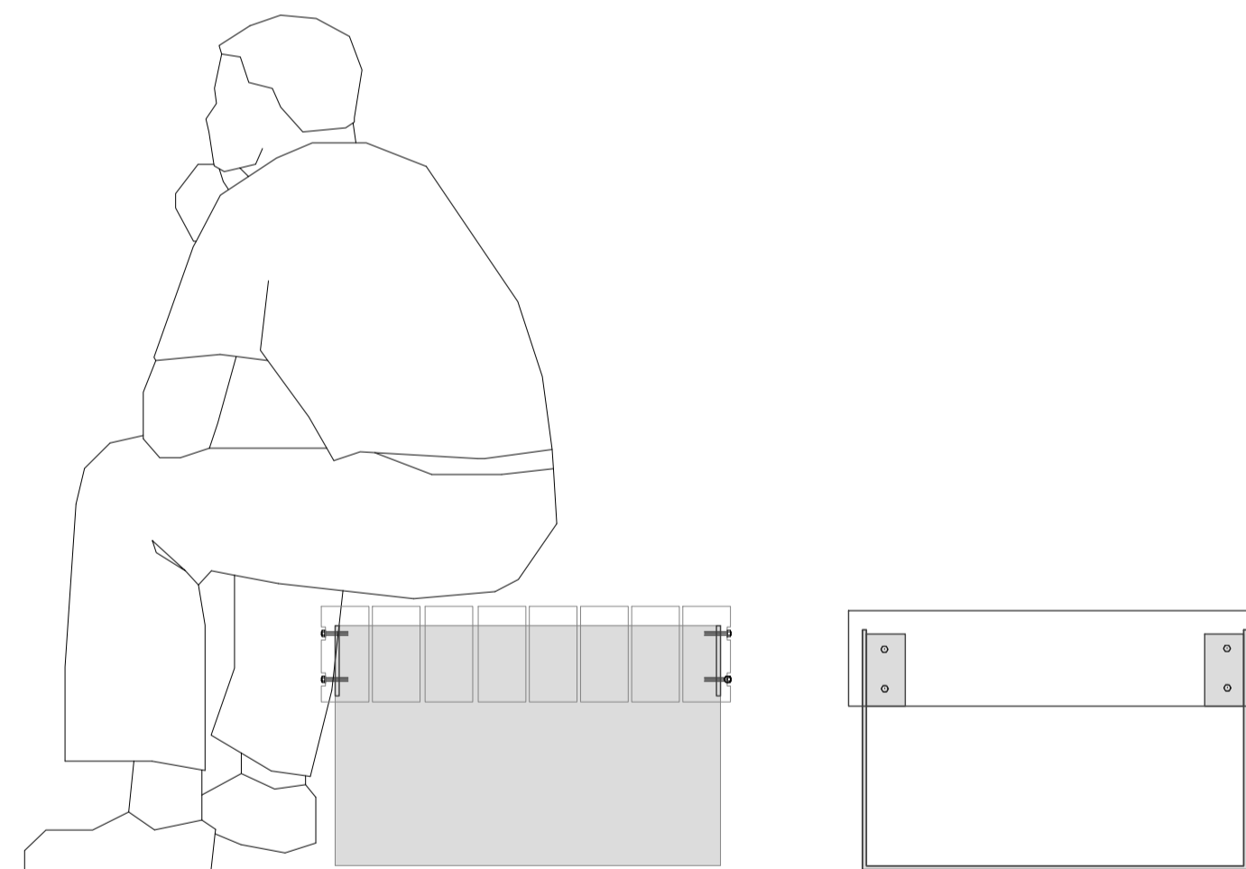
3 TYPICAL DETAIL: SEATING type b 12 SCALE 1:10 @ A1 Materials 6mm Corten steel Module 1 Hardwood Timber slats 140mm x 70 mm x 600
